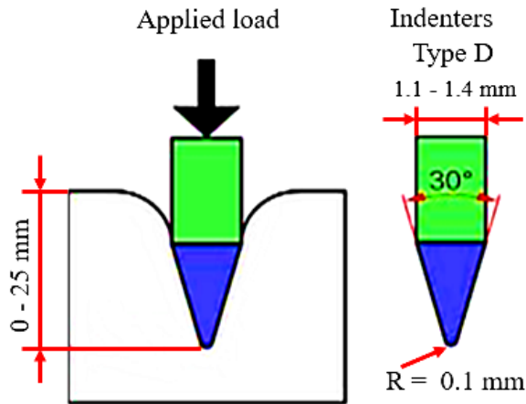
FIGURE.3. Shore D Test
